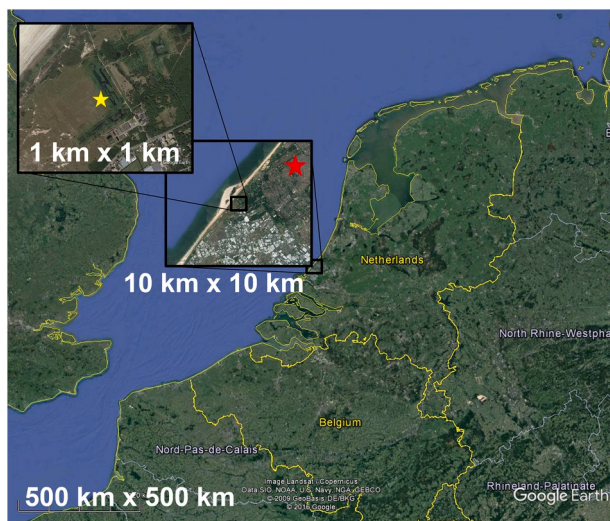
Fig. 1. Location of the measurement site in dune area Solleveld. The location of The Hague is marked with a red star in the 10 × 10 km inset, and the location of the GRAHAM instrument with a yellow star in the 1 × 1 km inset.
