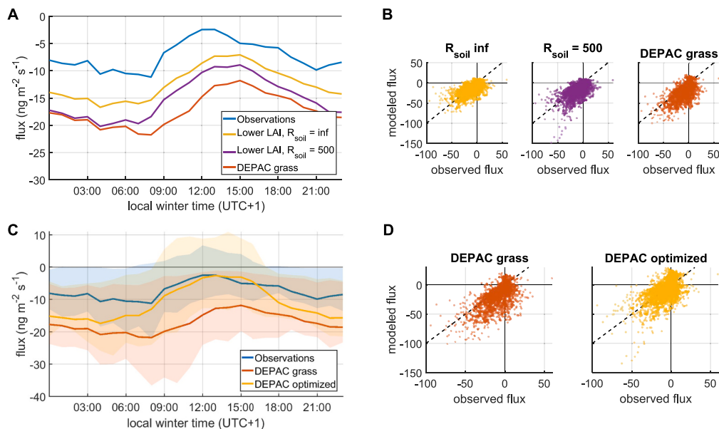
Fig. 8. (A,B) Diurnal variation (A) and scatterplots (B) of the DEPAC fluxes for standard grass settings ( LAI_{\min} = 2 ; LAI_{\max} = 3.5 ) compared with a lower LAI ( LAI_{\min} = 0.5 ; LAI_{\max} = 1 ), yet no exchange with the soil (yellow) and lower LAI combined with a finite soil resistance of 500 s/m (purple). (C,D) Diurnal variation with the 25/75 percentiles (C) and scatterplots of DEPAC fluxes in \text{ng m}^{-2} \text{ s}^{-1} (D), both plots compare the standard grass settings in DEPAC (red) and a run with lower LAI LAI_{\min} = 0.5 ; LAI_{\max} = 1.0 , R_{\text{soil}} = 500 \text{ s/m} , T_{\min} = 1^\circ \text{C} , T_{\text{opt}} = 18^\circ \text{C} , 2x higher \gamma_{\text{stom}} and 1.5x higher \gamma_w (yellow).
