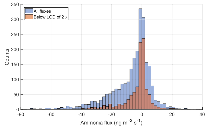
Fig. 9. Distribution of the ammonia fluxes. In blue are all measured fluxes, in red the subset that was not significantly different from zero because the concentration difference was below the LOD of 2\sigma .
